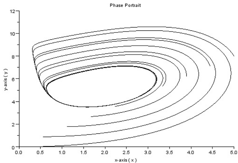
Figure 8.9: Oscillating Chemical Reactions
