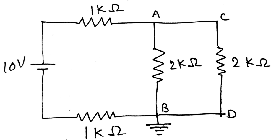
Circuit Diagram For Experiment 5
